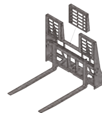
Standard Skid Steer with Walk Thru Brick Guard
